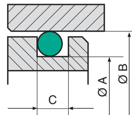
Tenuta pistone Piston application
